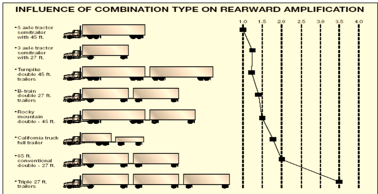
Figure 6.1 Rearward Amplification
