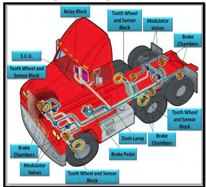
Figure 5.4 ABS System
