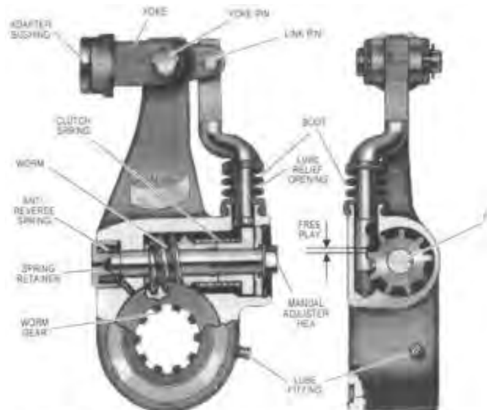
Automatic Slack Adjuster
