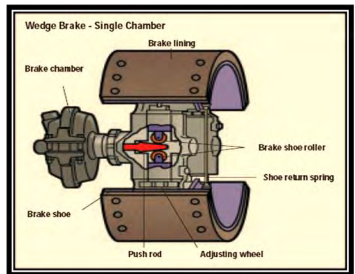
Figure 5.2a Wedge Brake
